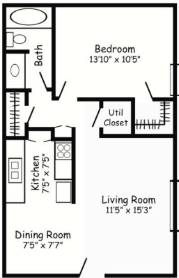
One Bedroom Apartment 633 sq ft
